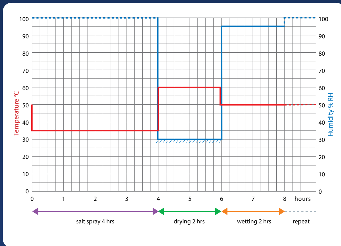
CETP 00.00-L-467 (Ford/Volvo ACT-2, VCS1027,1449, TP/LR-52-265)
